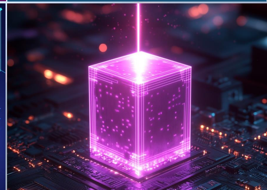
Quantum Computing
